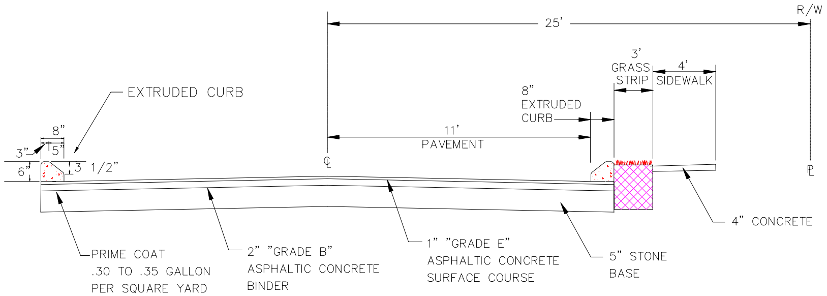
TYPICAL SECTION - RESIDENTIAL
